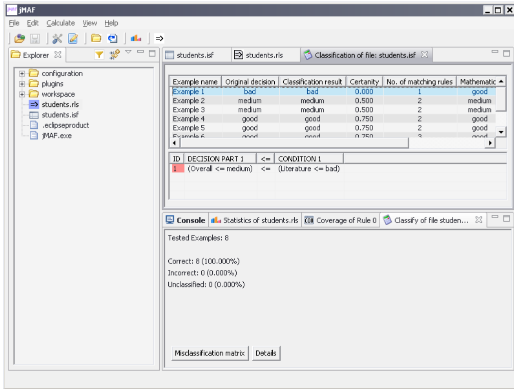
Figure 15: Details of classification
