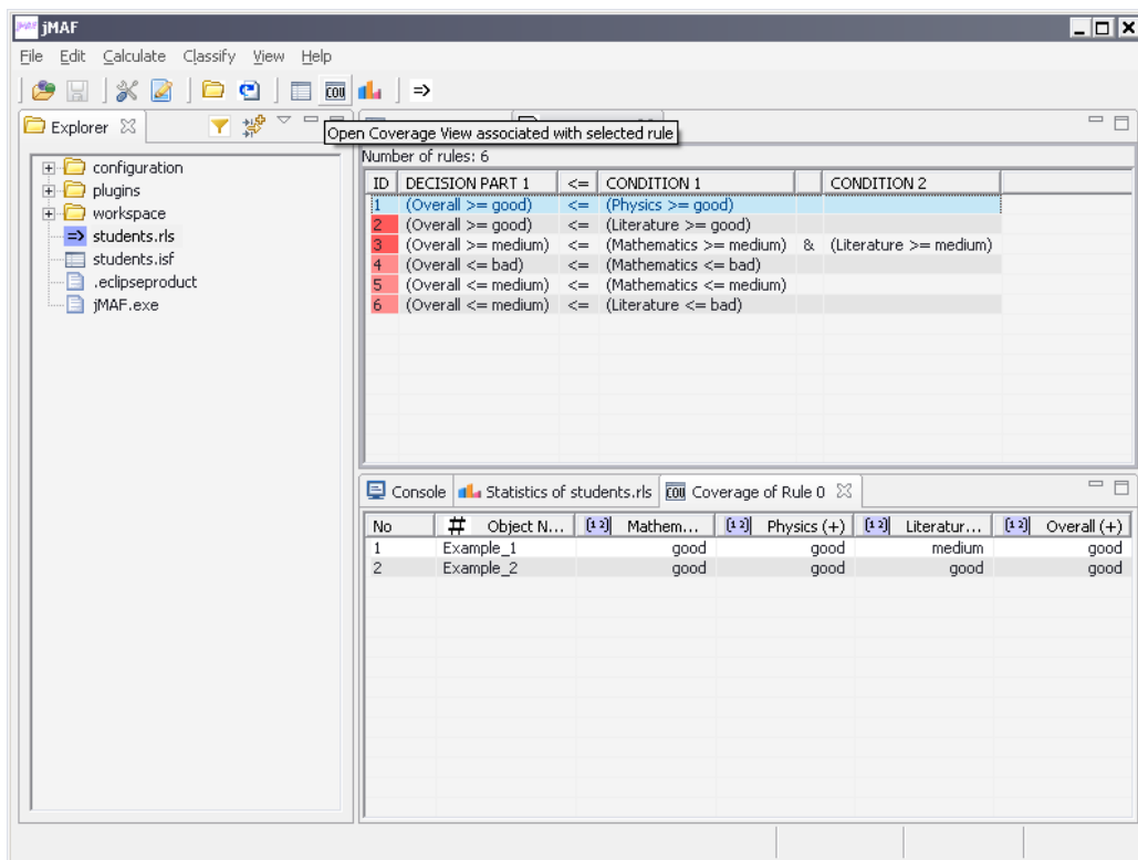
Figure 12: Coverage of the first decision rule
