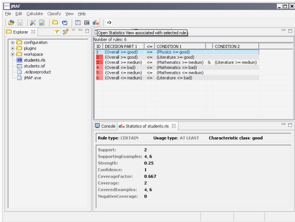
Figure 11: Statistics of the first decision rule
