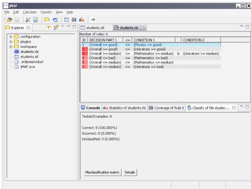
Figure 14: Results of classification
