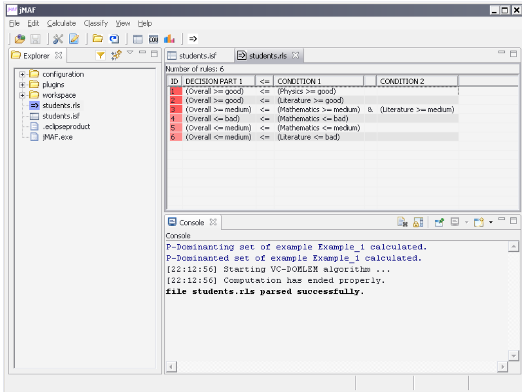
Figure 10: Decision rules
