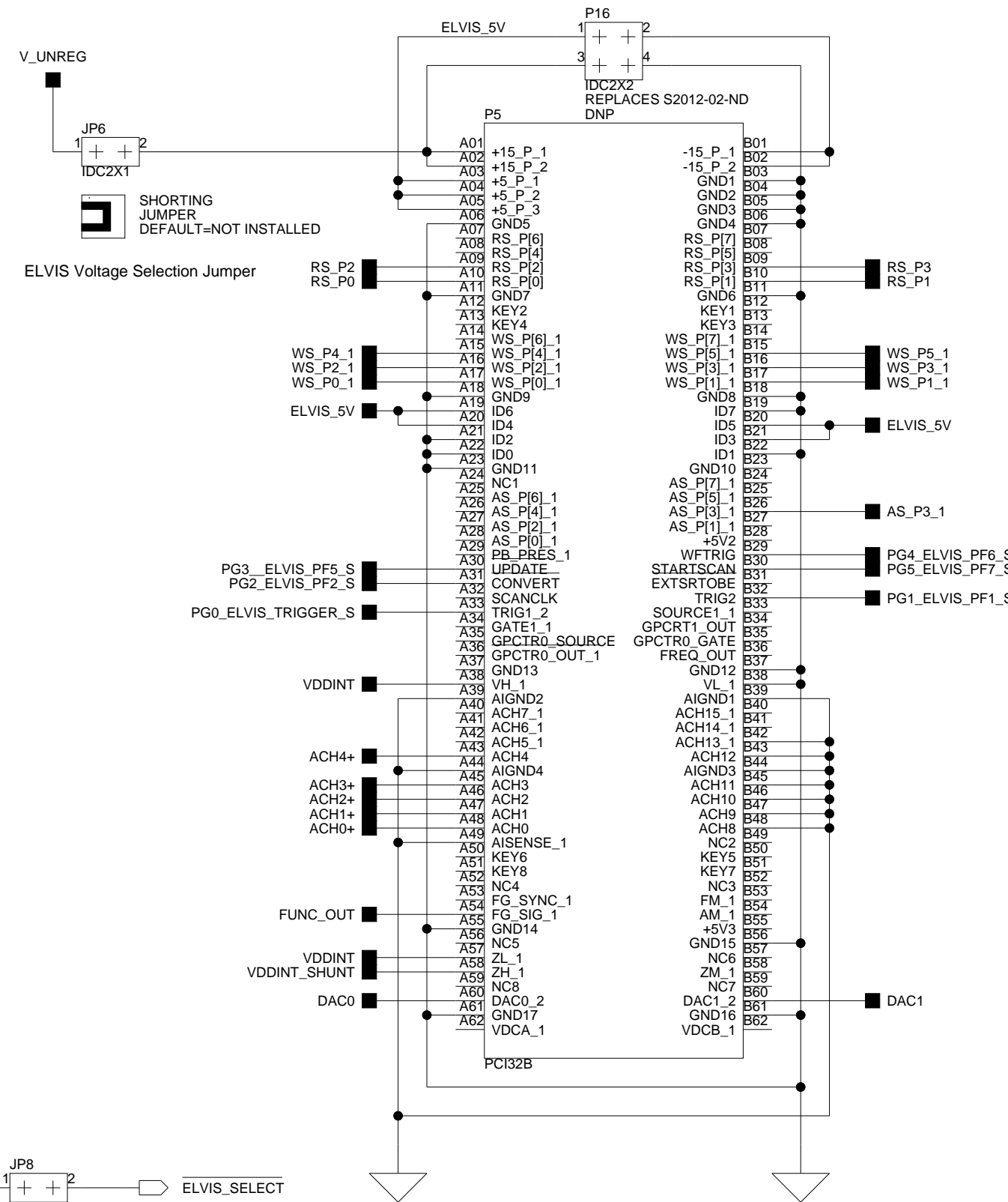
ELVIS CONNECTOR
