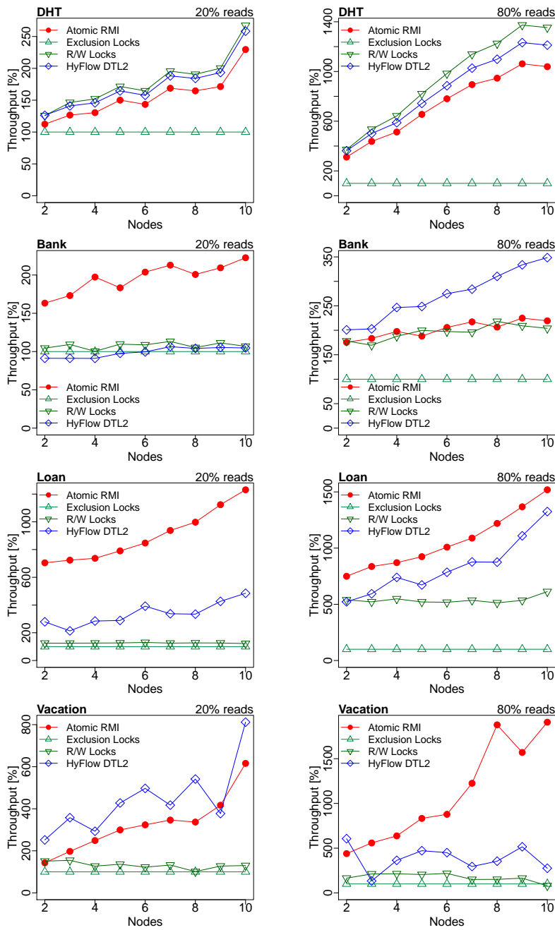
Fig. 13: Evaluation results by benchmark (DHT, Bank, Loan, and Vacation) and read/write transaction ratio (20% reads vs 80% reads). Each benchmark is presented on two graphs: one for 20–80 read/write operation ratio, and the other for 80–20 ratio. Points on the graph represent the mean throughput (on the y-axis) from the given benchmark run on a particular number of nodes (on the x-axis). The results are shown as a percentage improvement in relation to the execution of Exclusion Locks.
