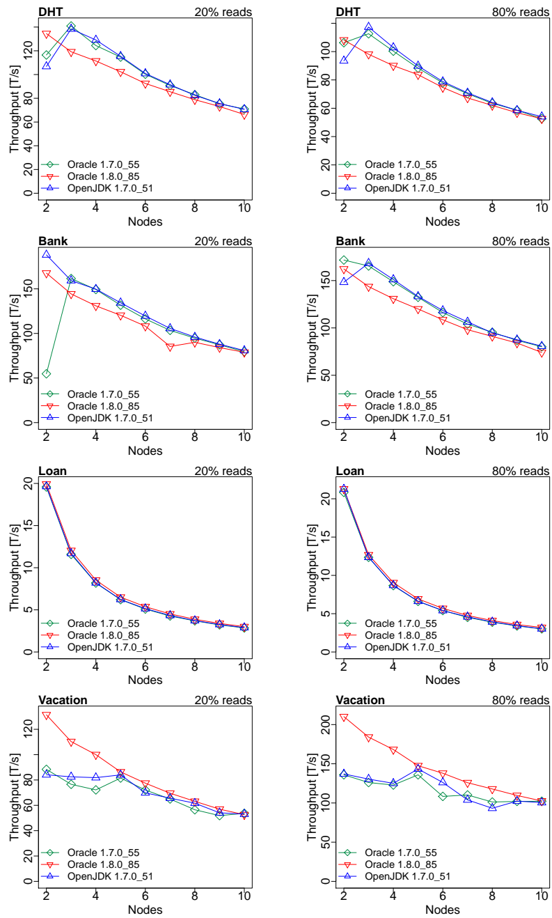
Fig. 14: Evaluation results of Atomic RMI under various JREs. Points on the graph represent the mean throughput in transactions per second (on the y-axis) from the given benchmark run on a particular number of nodes (on the x-axis).
