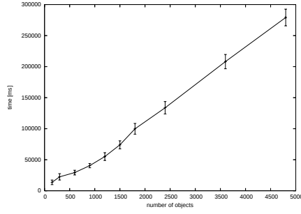
Fig. 4. time vs. number of objects
