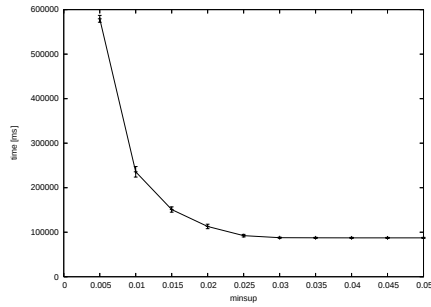
Fig. 6. time vs. minsup
