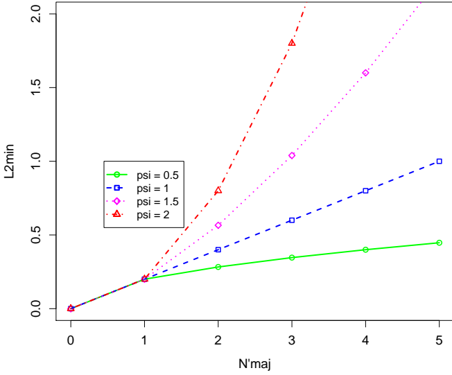
Figure 1: L_{min}^2 weights depending on \psi .
