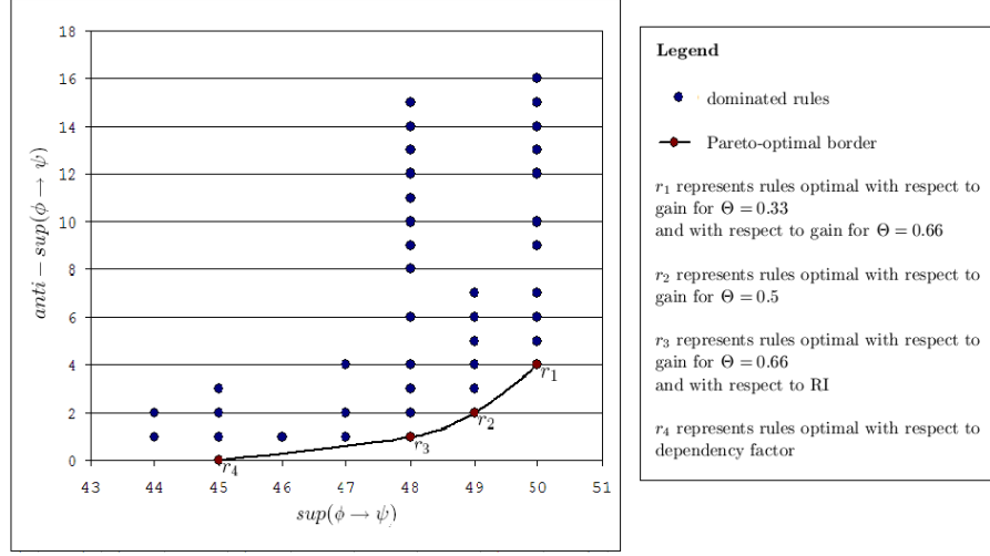
Figure 2. Pareto-optimal border with respect to rule support and anti-support includes rules being optimal in RI , and gain
