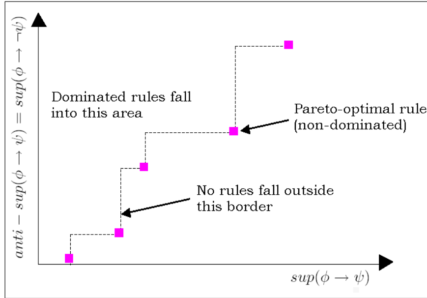
Figure 1. Support-anti-support Pareto-optimal border
